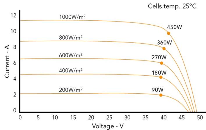
TYPICAL I-V CURVES
