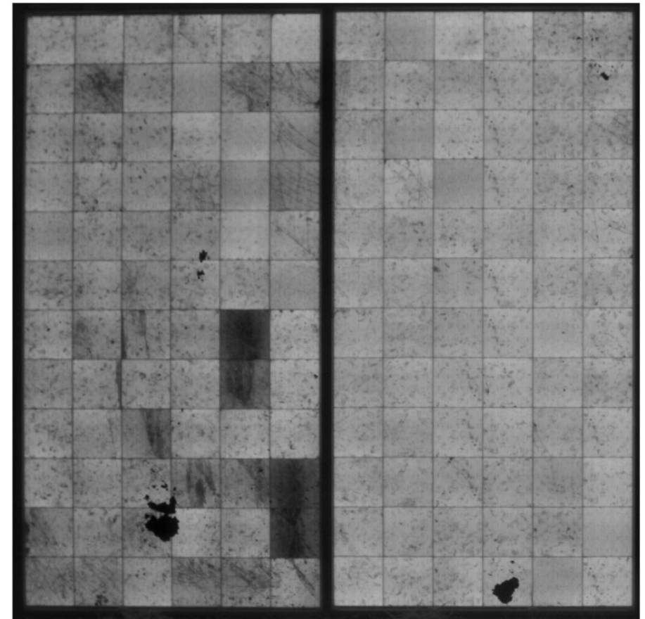
ELECTROLUMINESCENCE TEST
