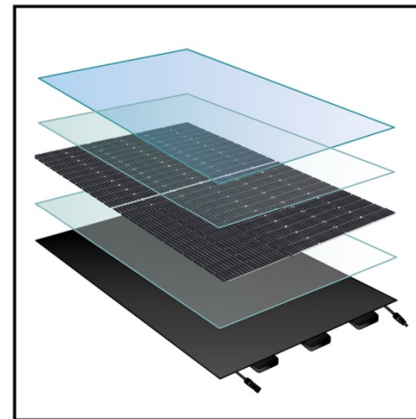
LAMINATION
